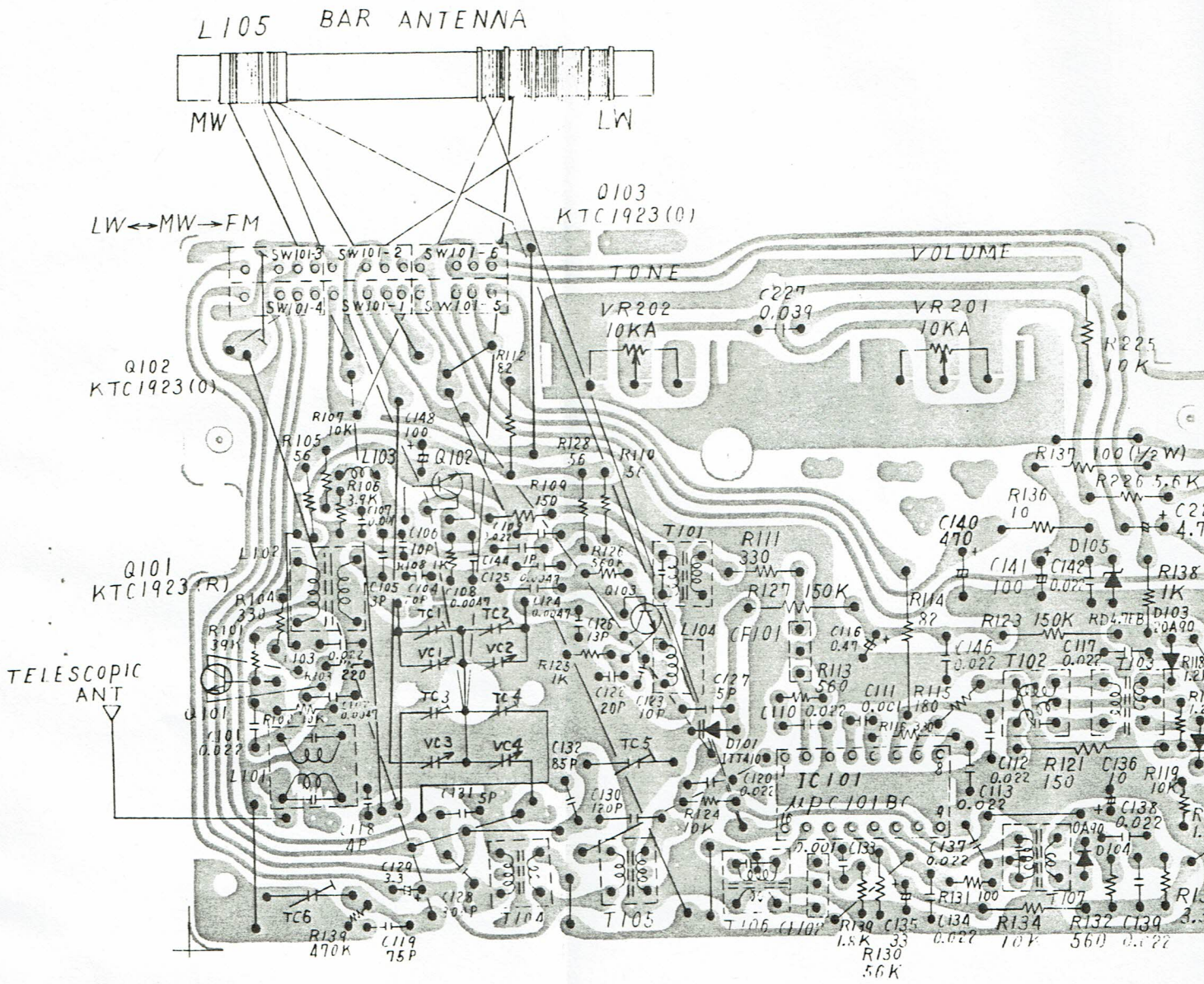
P.C.B. 1 TUP-229 Bottom View
